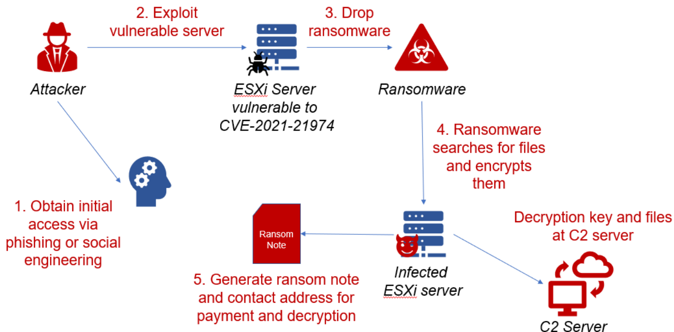
Figure 4 – Attack chain
